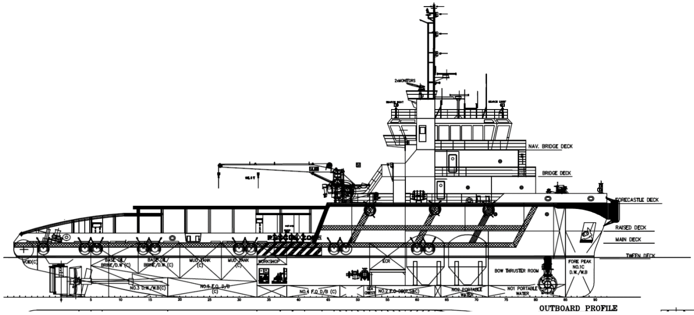
OUTBOARD PROFILE
