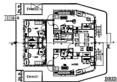
BRIDGE DECK
