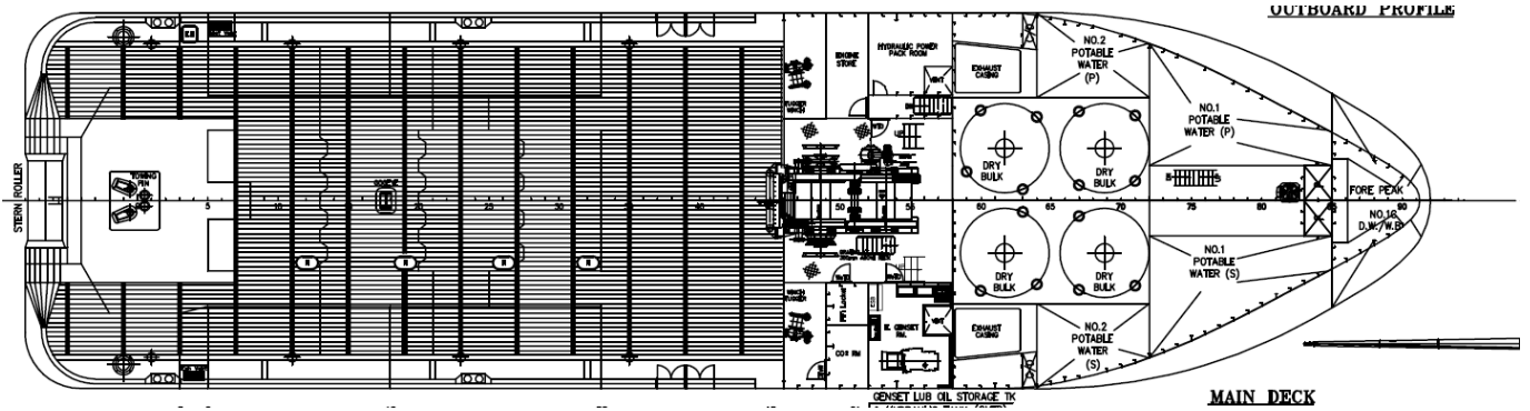
MAIN DECK
